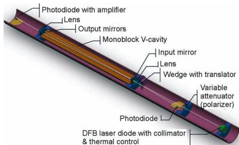
Fig. 3. General layout of the embedded OFCEAS spectrometer.
